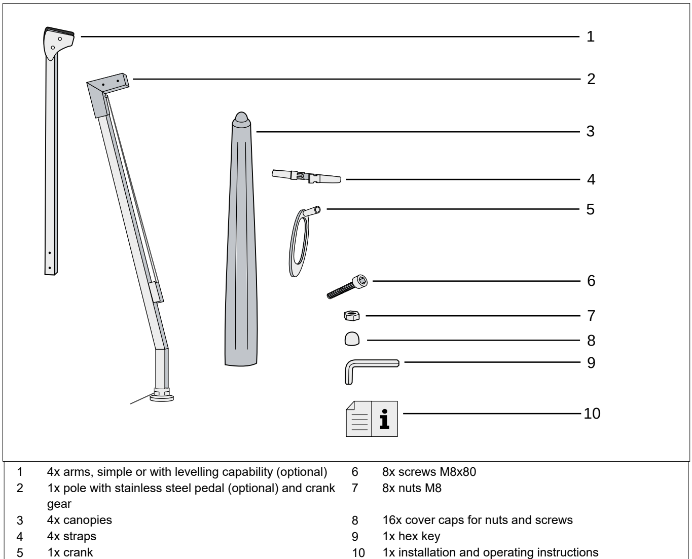
Fig. 7: Scope of delivery Amalfi Quadro
