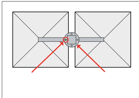
Fig. 8: Aligning the threaded holes of the DUO 1
